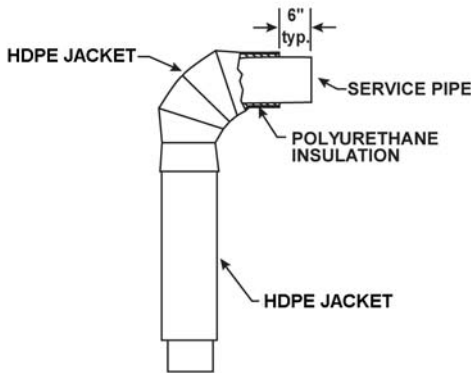
90° ELBOW WITH EXPANSION LEG FOR EXPANSION LOOPS
