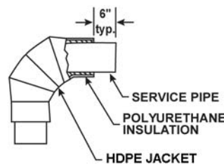
STANDARD 90° ELBOW FOR DIRECTION CHANGES
