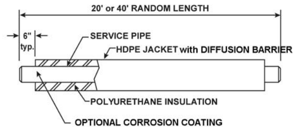
STRAIGHT STANDARD LENGTH
